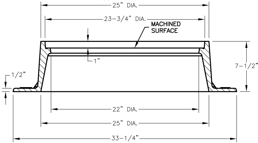
SECTION B-B
