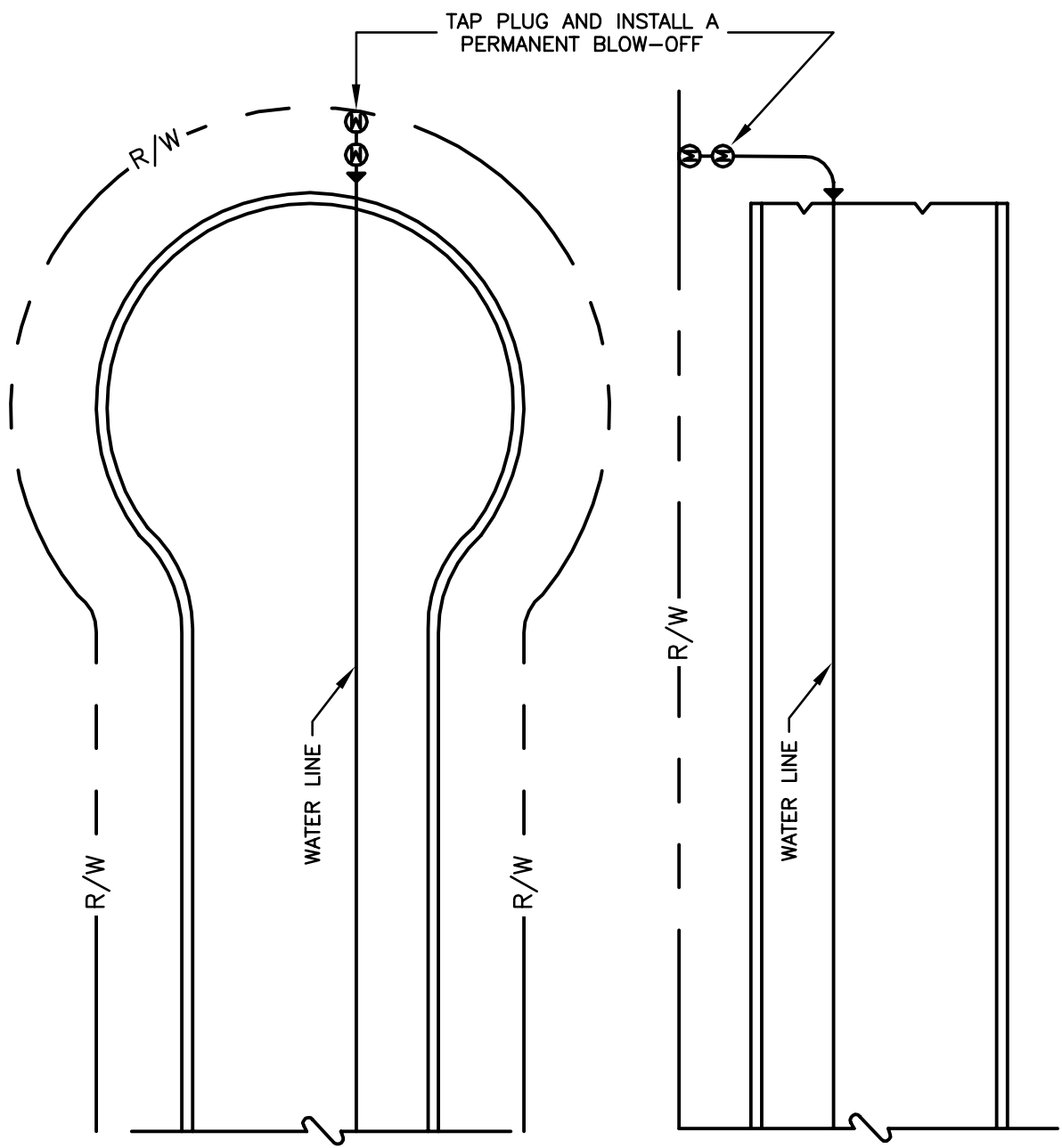
CUL-DE-SAC SET VALVE BOXES 2' OFFSET FACE OF CURB
