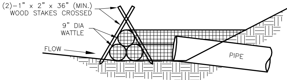
SECTION VIEW
