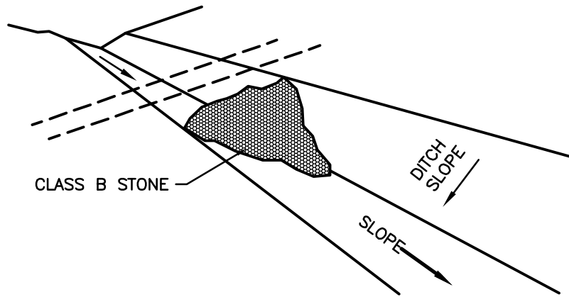
ISOMETRIC VIEW
